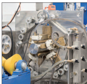
ECHOGRAPH-STPS bar testing system
