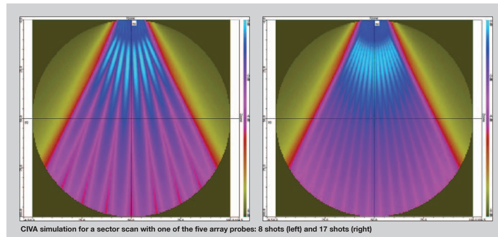
CIVA simulation for a sector scan with one of the five array probes: 8 shots (left) and 17 shots (right)
