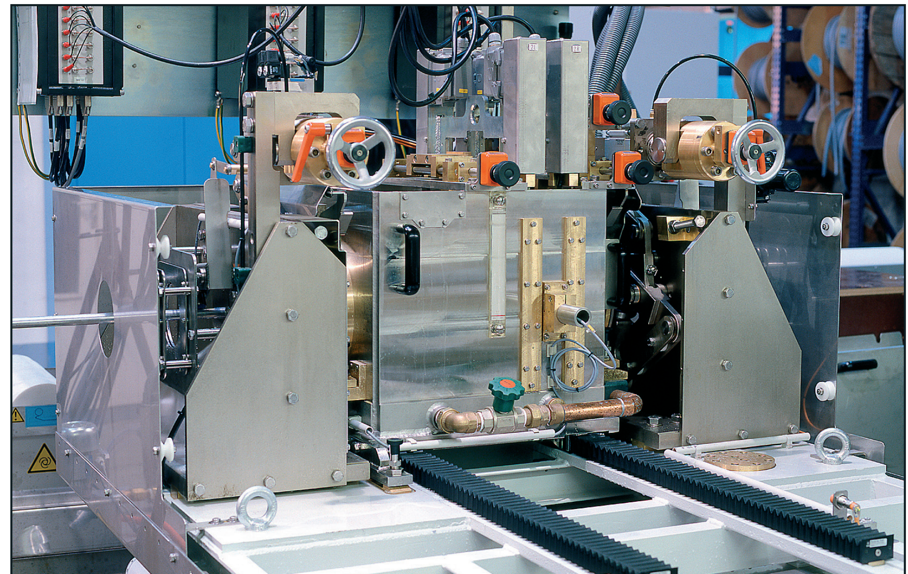
ECHOGRAPH-HRPS Bar Testing with Immersion Tank
