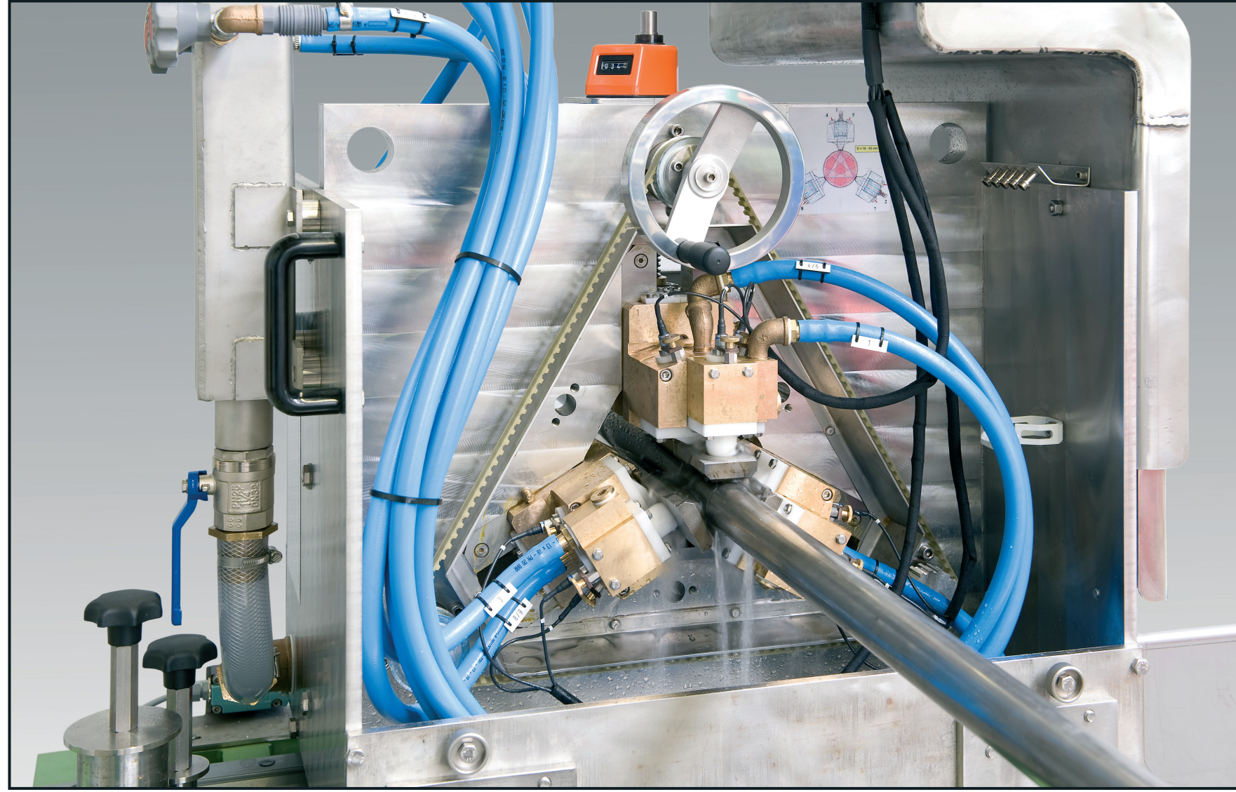
ECHOGRAPH-STPS Bar Testing with Squirter Coupling
