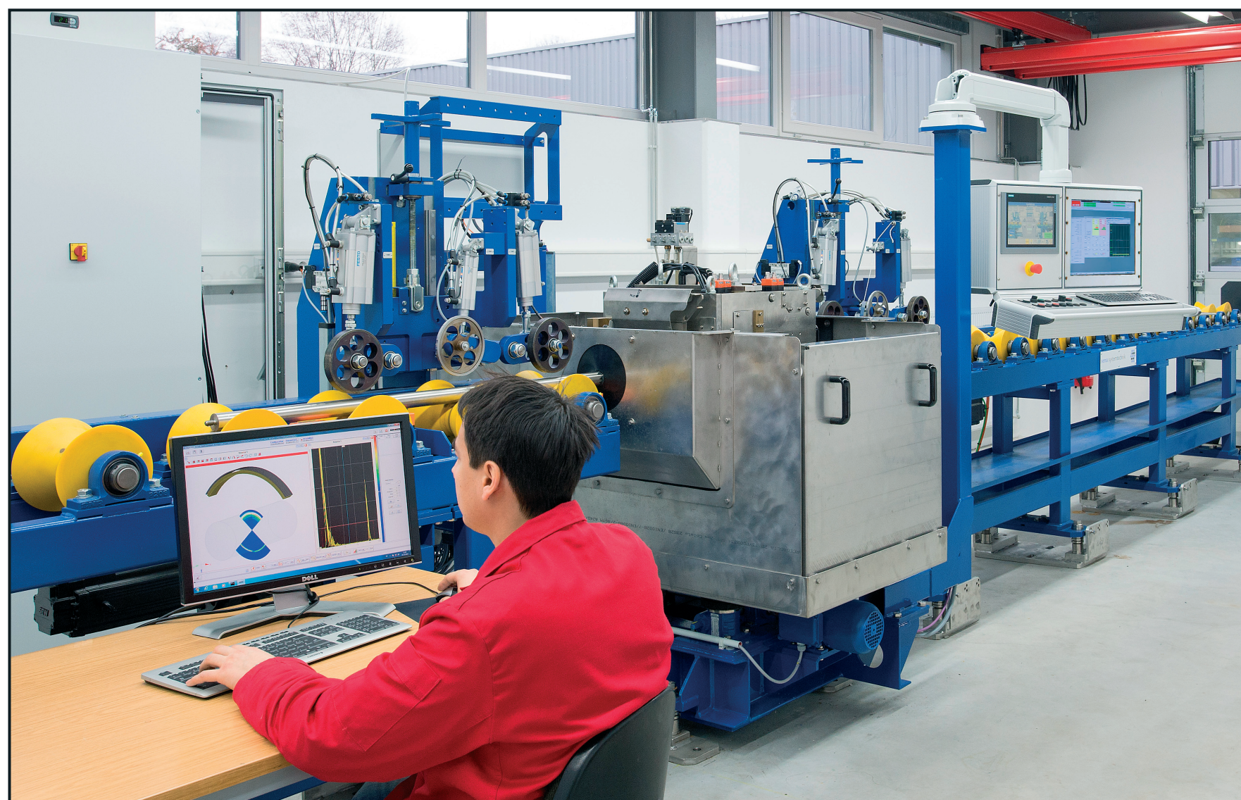
ECHOGRAPH-HRPS Phased Array Bar Testing
