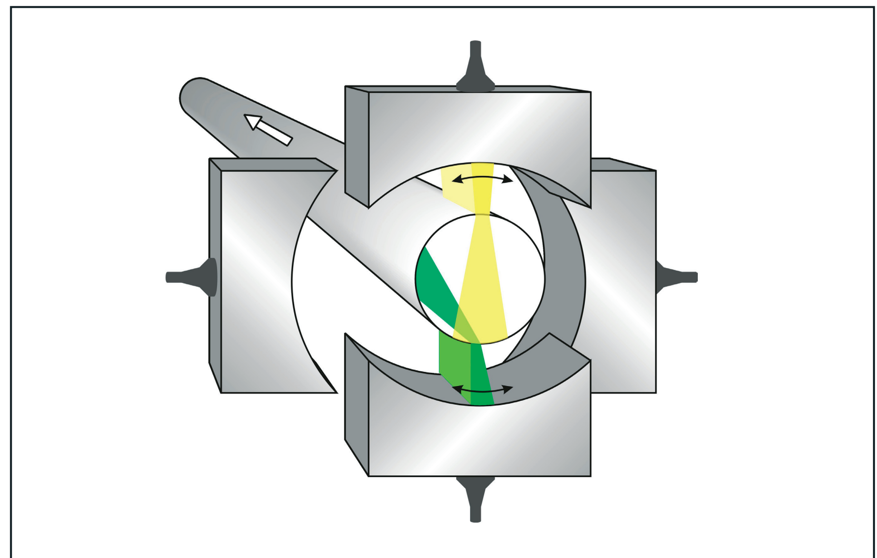
ECHOGRAPH-HRPS Testing Principle (4 Array Probes)
