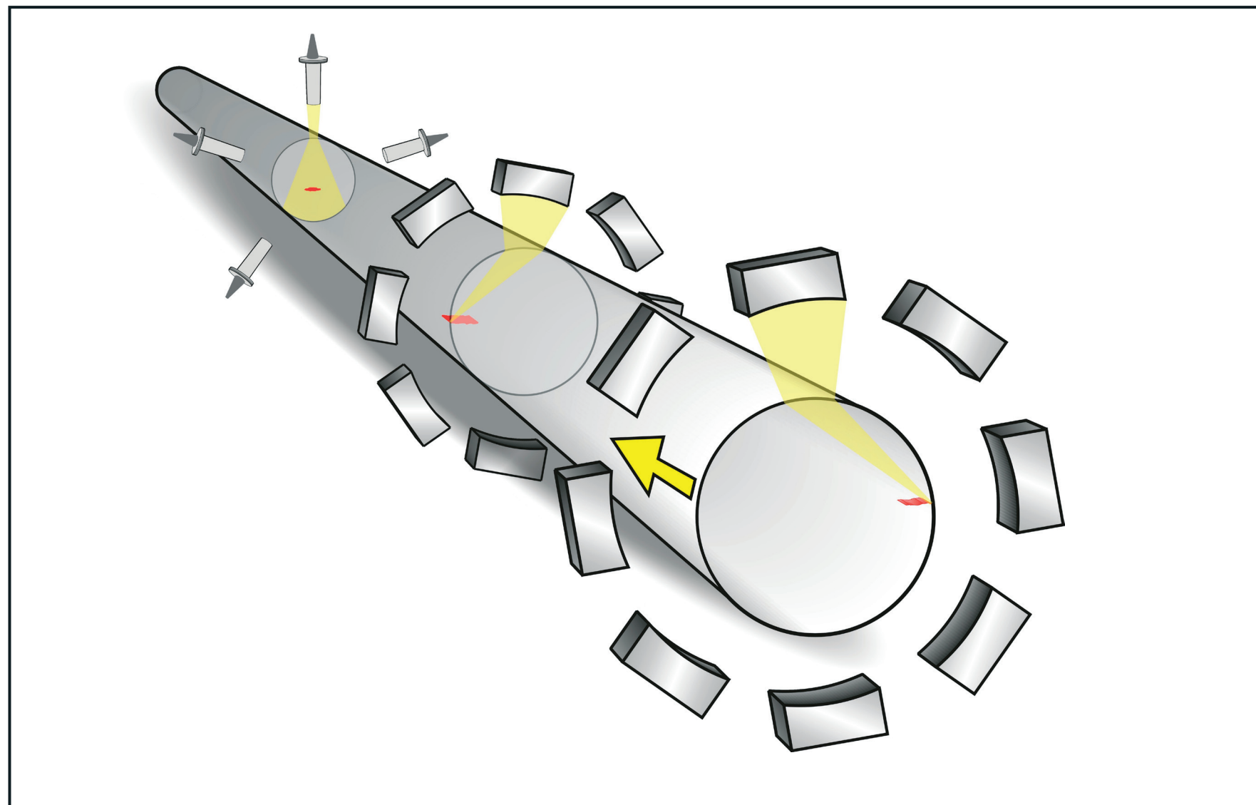
ECHOGRAPH-HRPS Testing Principle (21 Probes)
