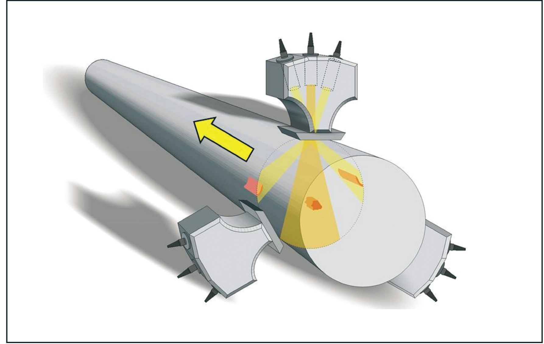
ECHOGRAPH-STPS Testing Principle (9 Probes)
