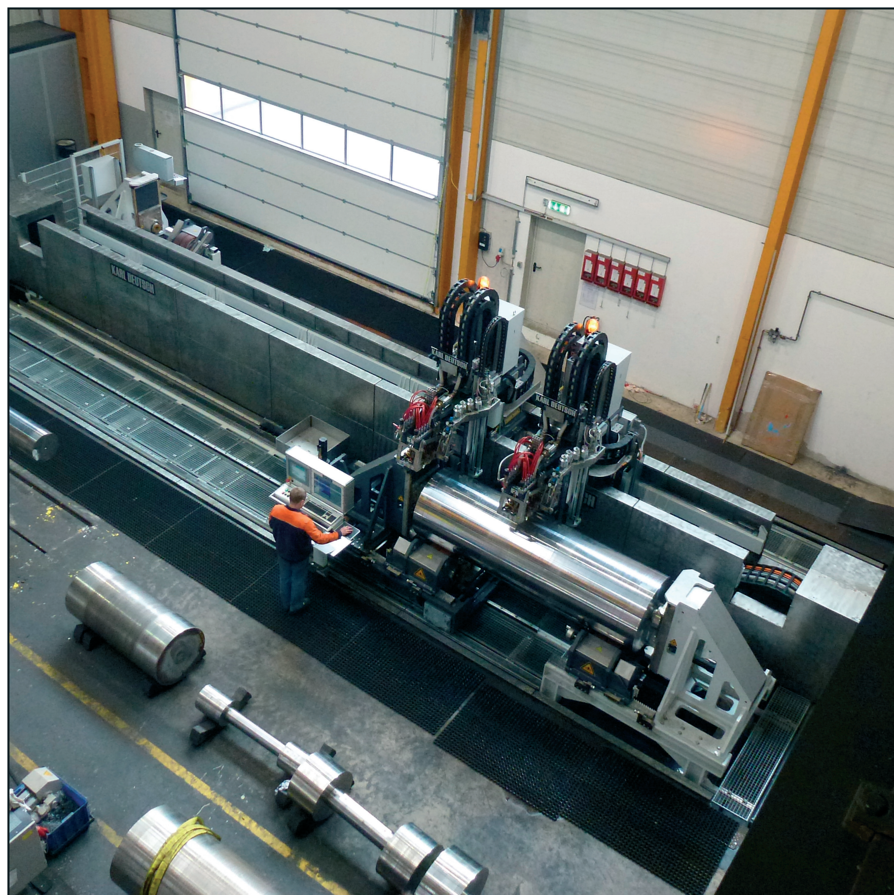
Testing Portal with Two Stations
