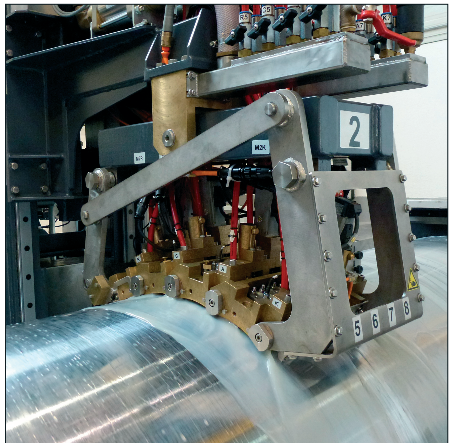
32 Probes Mounted into Two Probe Holders
