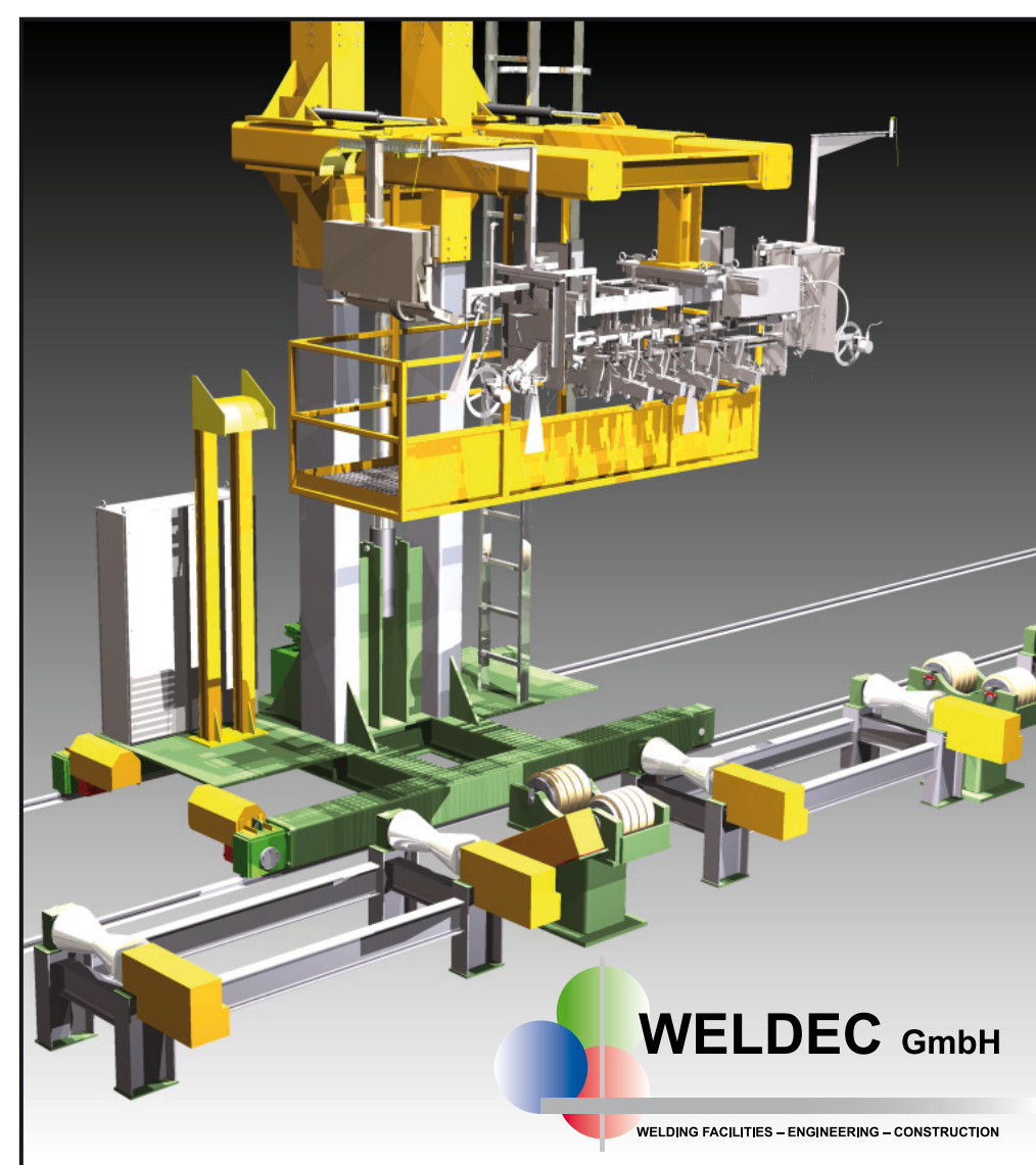
WELDEC Machine Stand and Pipe Conveyor
