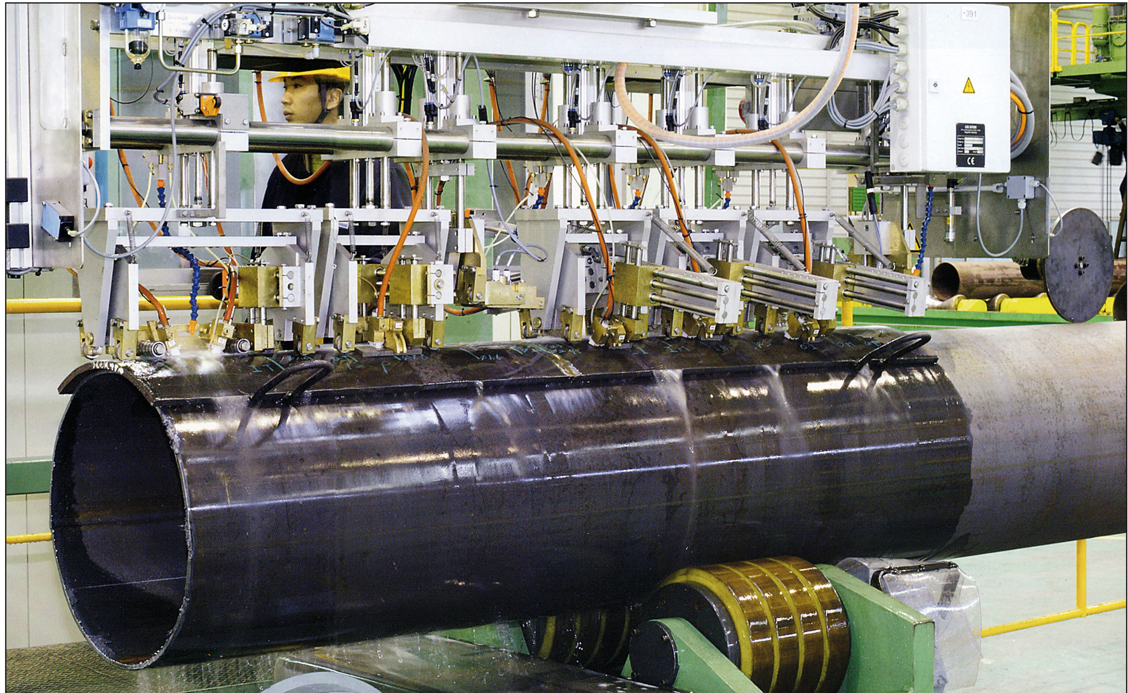
Probe Holders for Longitudinally Welded Pipe Testing @ EEW-Korea
