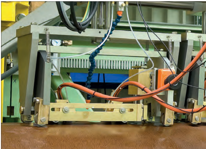
Probe holders for the on-bead detection of transverse defects: Water jet coupling enables positioning of the probes directly on the weld crown.
