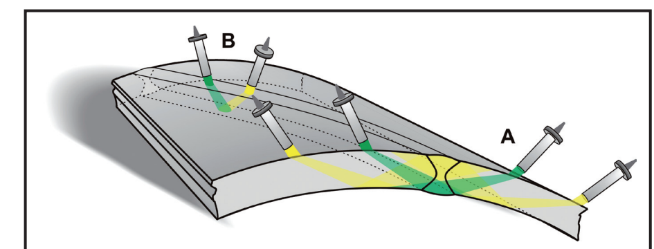
First ultrasonic weld test, 6 angle beam probes
