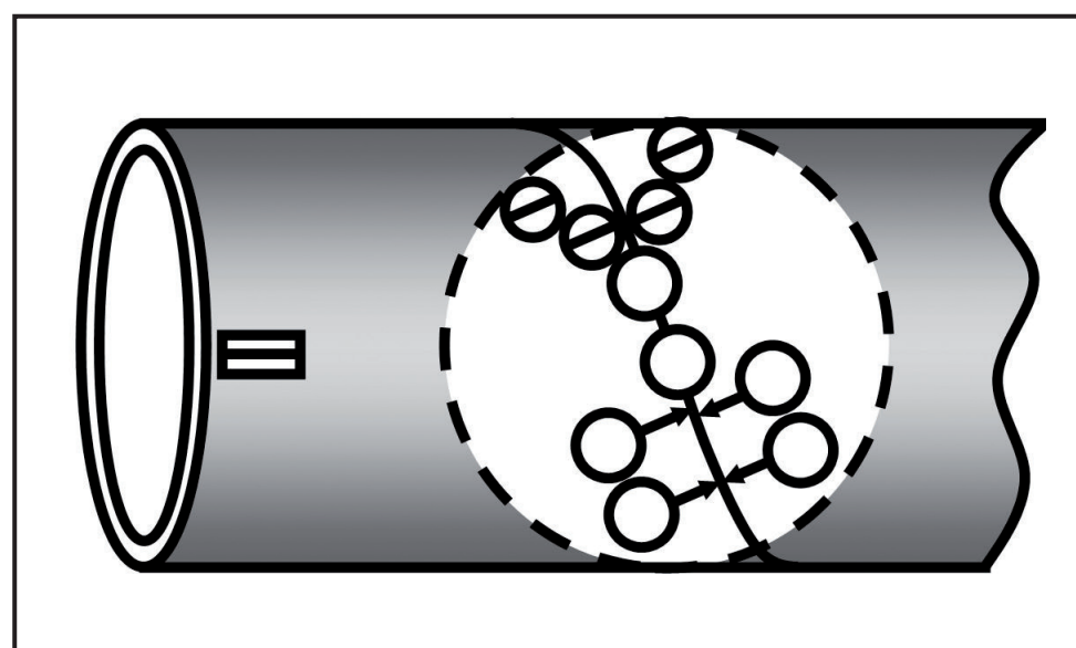
SNUS probe configuration for final ultrasonic test
