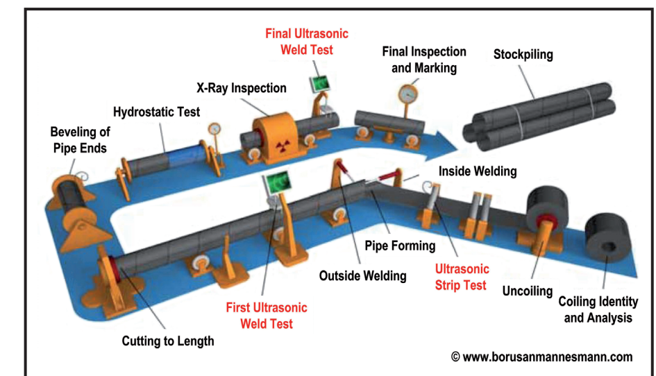
Production and testing of HSAW pipes
