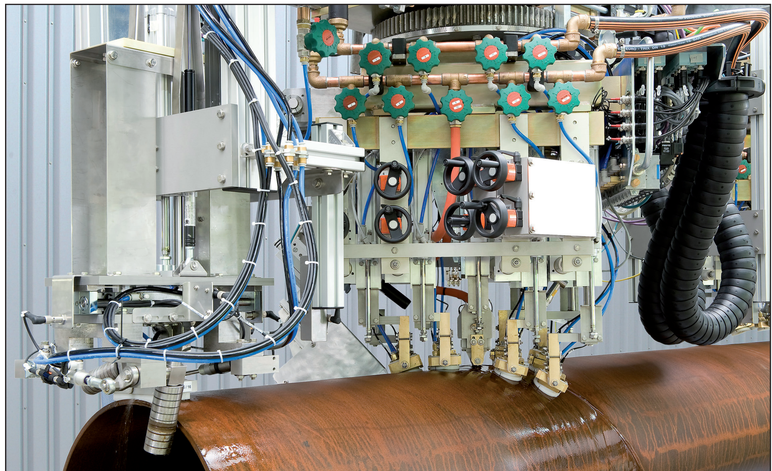
SNUS final ultrasonic weld and pipe end testing system: 11 probes in 2 separate frames
