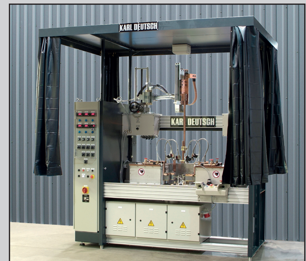
Machine with darkening cabin
