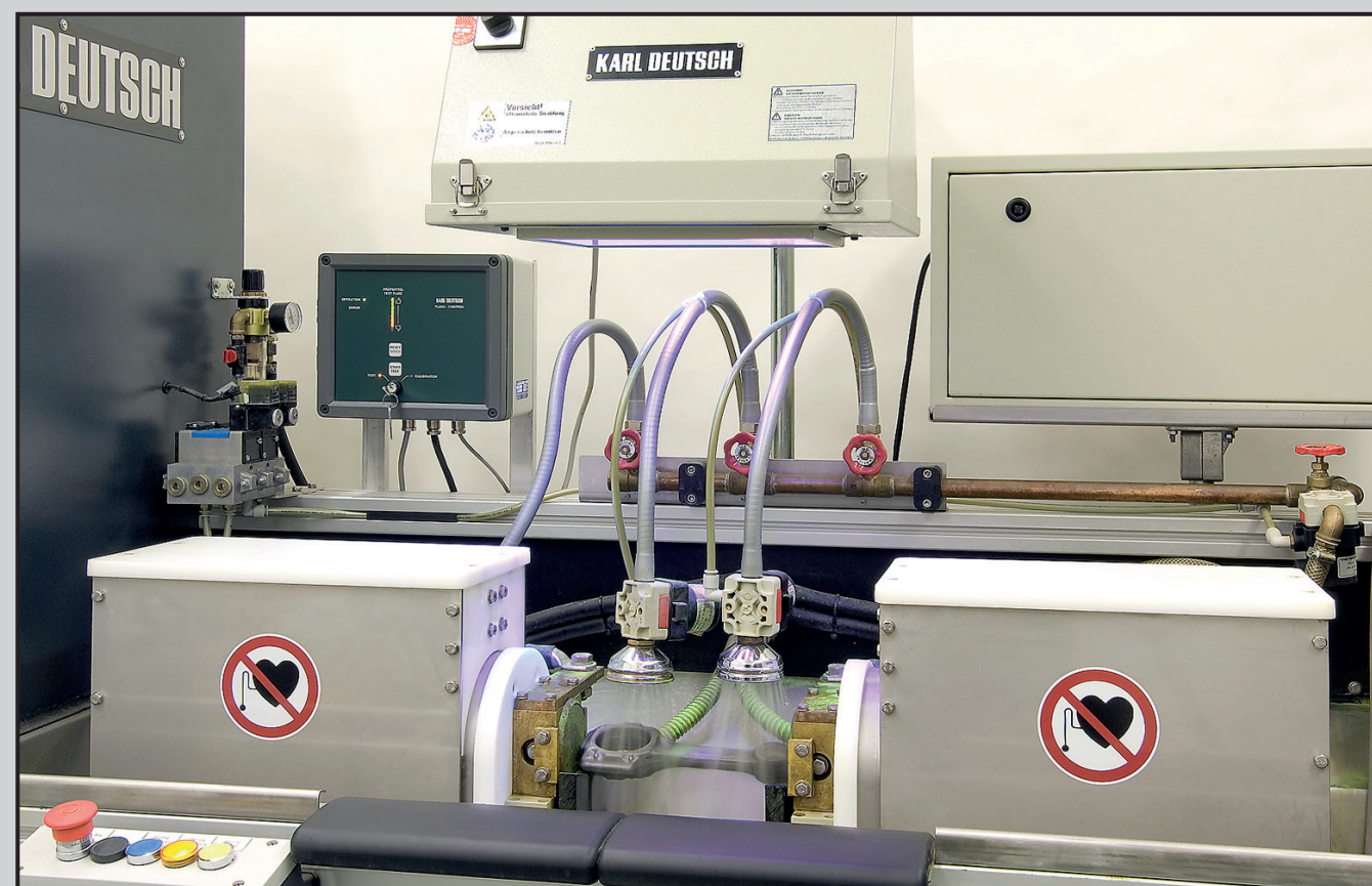
FLUXA-Control for automatic supervision of inspection fluid
