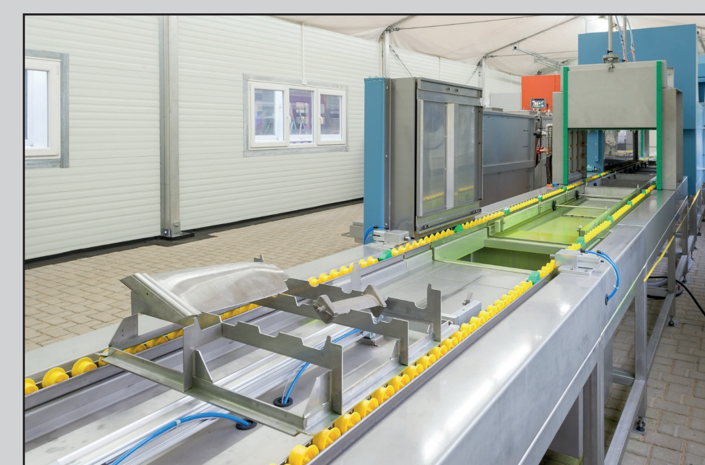
Fully-Automated Penetrant Testing of Forgings
