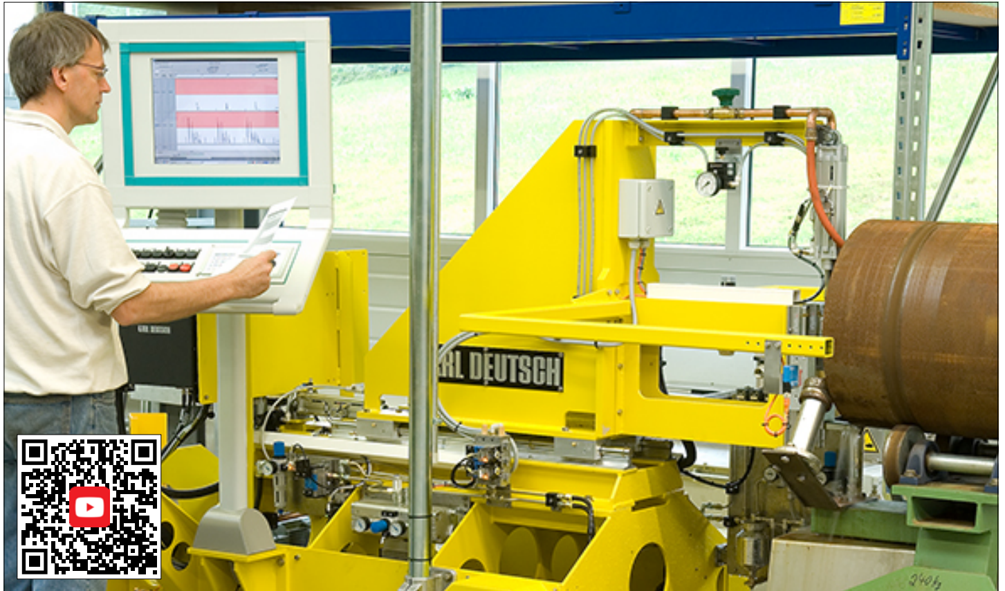
Entering the test parameters and checking the calibration of the testing system
