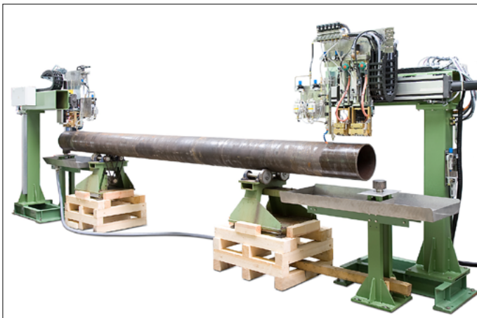
Two machine stands – one for each tube end and provisional tube rotating device for assembly at KARL DEUTSCH systems workshop
