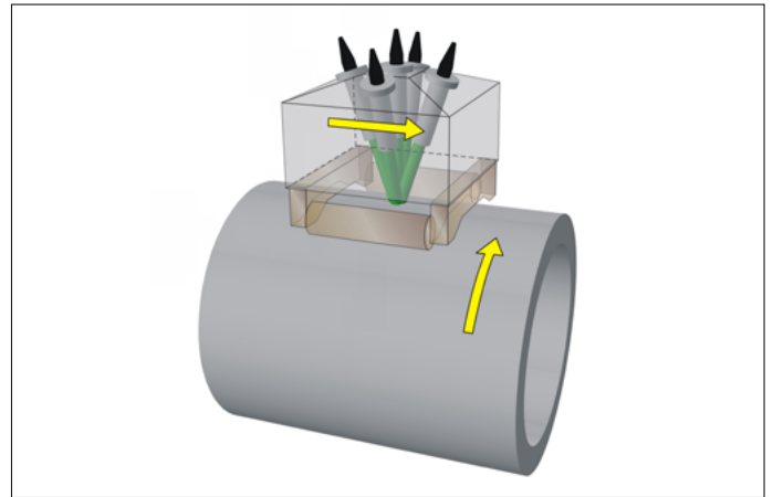
Testing principle with five ultrasonic probes and helical testing traces (rotating tube, linear movement of probe holder, probe holder in 12 o'clock position). Longitudinal defects are detected with two probes which transmit ultrasound in both circumferential directions (clockwise, counter-clockwise). Transverse defects are detected with two probes with ultrasonic incidence in the tube axis direction. One straight beam probe is used to measure the wall thickness and for lamination detection.
