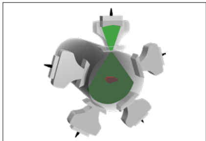
Testing principle (5 arrays): sector scan for each array
