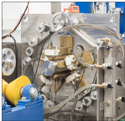
ECHOGRAPH STPS bar testing system
