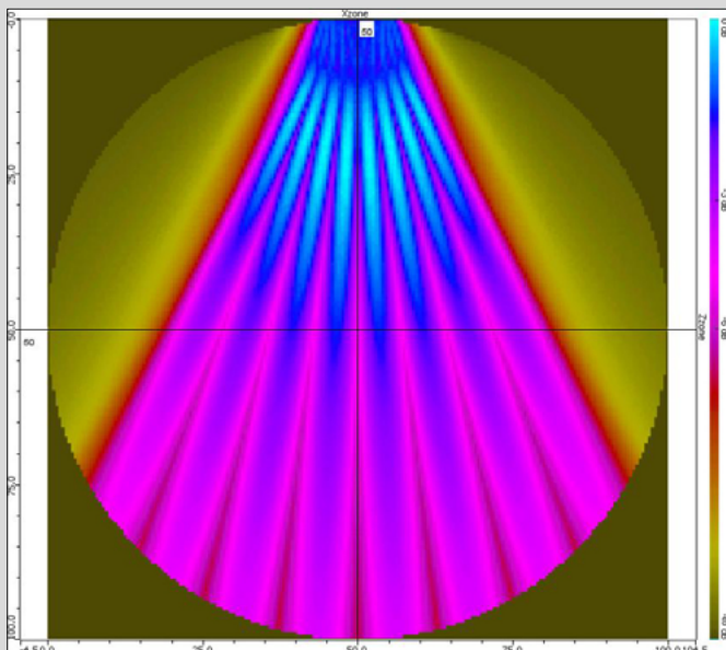
CIVA simulation for a sector scan with one of the five array probes: 8 shots (left) and 17 shots (right)
