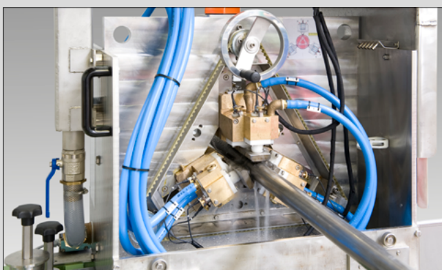
The STP-system works with three probe carriers (couplant wipers and protection housing of the system are dismantled in this picture). Each probe carrier accommodates one probe for normal incidence. Two angle beam probes can also be integrated in each probe carrier for detection of surface-near flaws.
