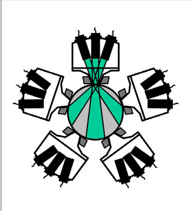
Optional probe configuration with 15 probes
