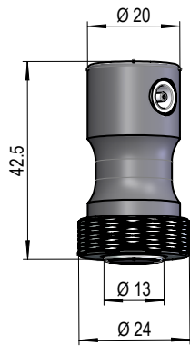
Housing S 10
