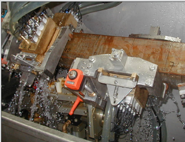
Four probe holders for quadratic billets, each carrier with seven probes and positioning from all four sides. The guidance is achieved by guiding rollers and hard-metal skids.
