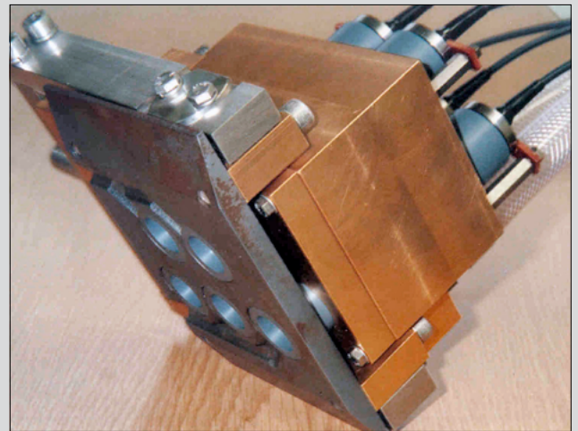
Probe holder for quadratic billets. The ultrasonic coupling is achieved by guided water jets (squirtter technique).
